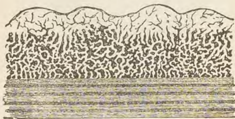
SECTION OF SCALE OF HOLOPTYCHIUS.
